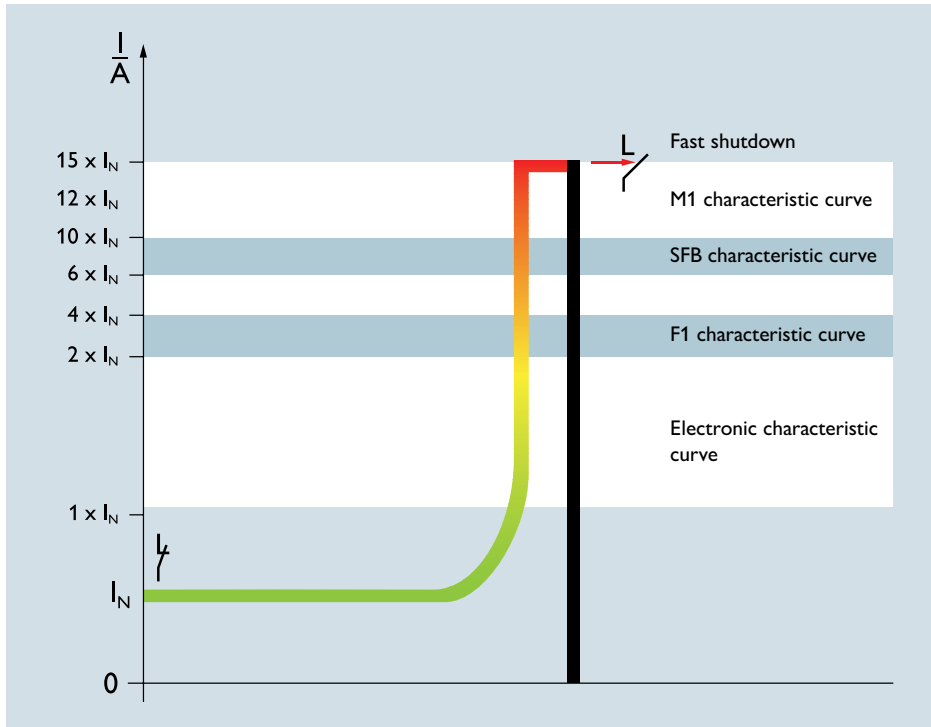
Tripping behavior of various device circuit breakers
