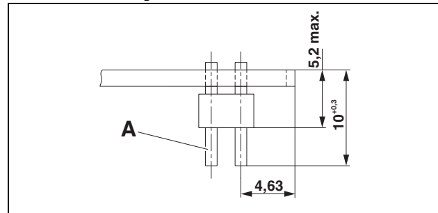
Figure 60 Dimensional drawing of connector on perpendicular PCB (all except for BC 17,8) for contacting in the DIN rail connector
