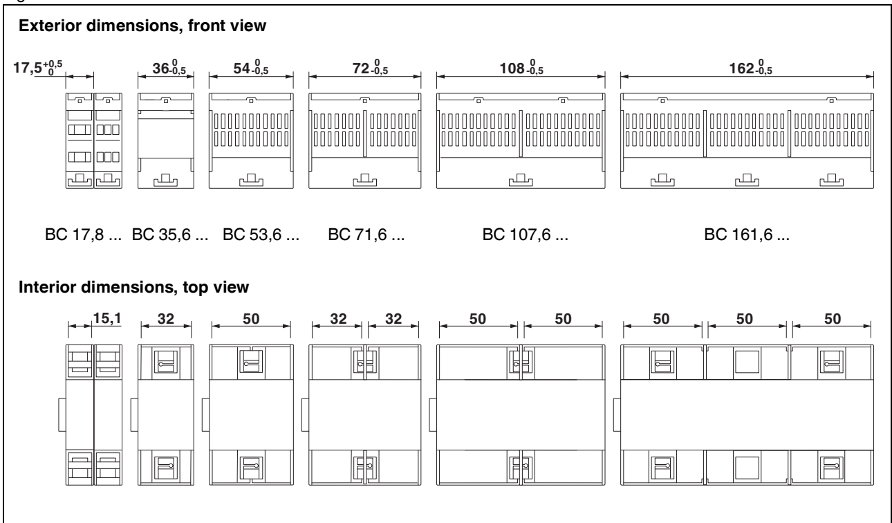
Figure 7 Exterior and interior dimensions
