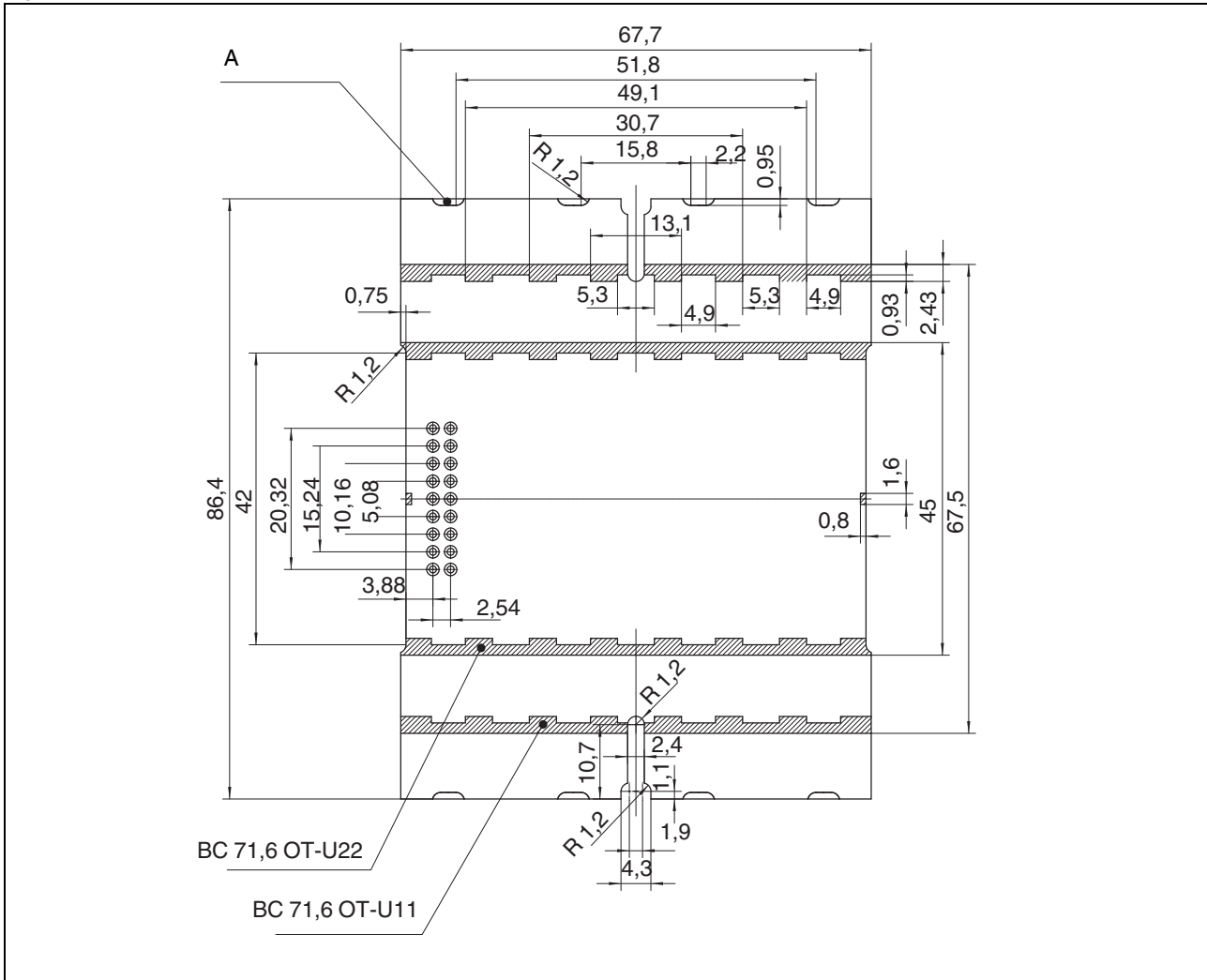
Figure 19 Dimensions of PCB 1 (BC 71,6) – upper side
