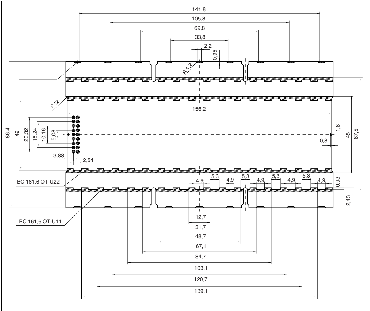
Figure 23 Dimensions of PCB 1 (BC 161,6) – upper side
