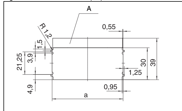
Figure 41 Dimensions for perpendicular PCBs
