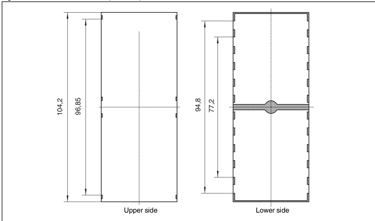
Figure 35 Dimensions of PCB 9 (BC 107,6)
