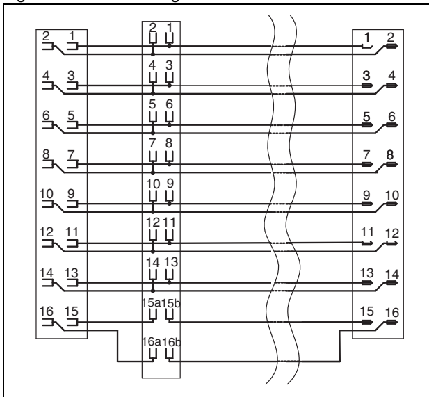
Figure 59 Circuit diagram HBUS...-16P-1S BK
