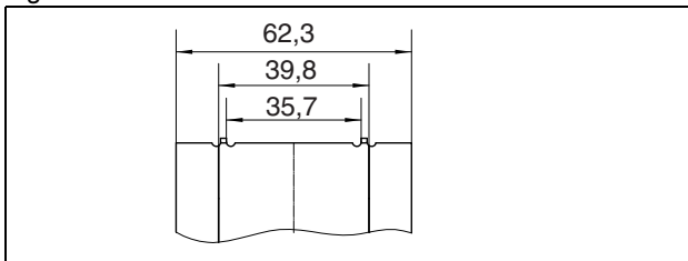
Figure 26 Dimensions of PCB 3
