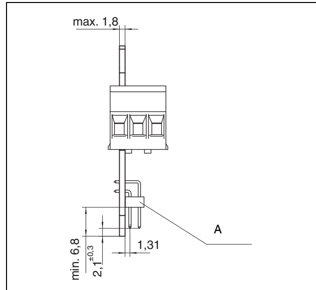
Figure 14 Dimensional drawing of connector on perpendicular PCB (in BC 17,8) for contacting in the DIN rail connector
