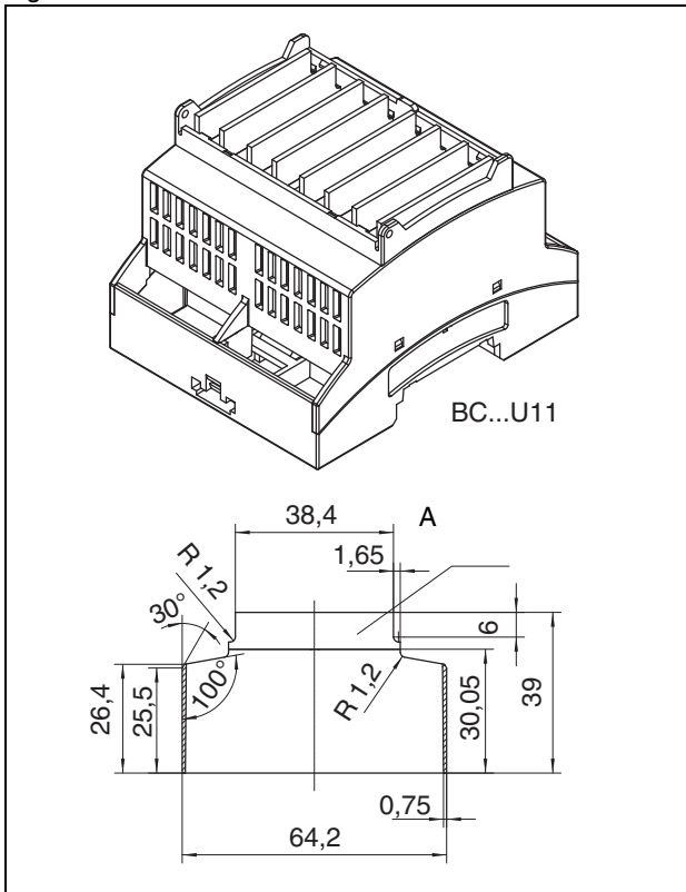
Figure 37 Dimensions of BC...U11
