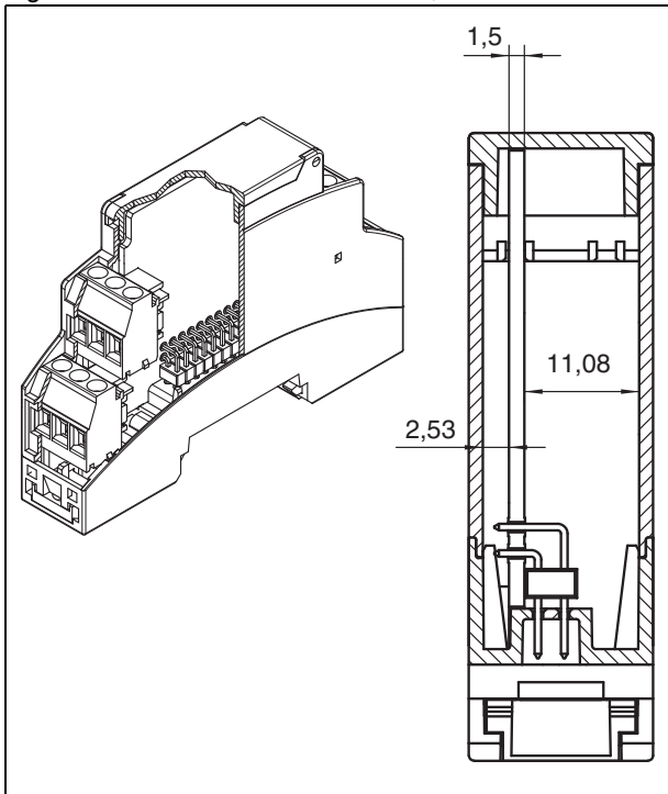
Figure 11 Inner dimensions BC 17,8
