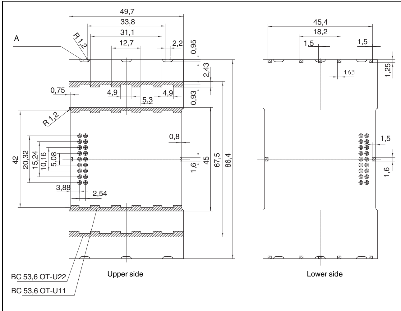
Figure 18 Dimensions of PCB 1 (BC 53,6)
