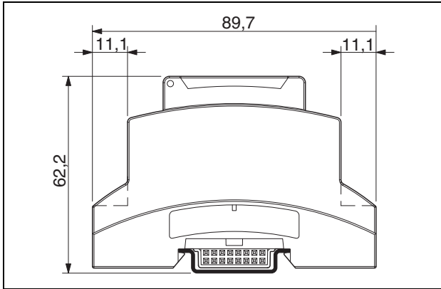
Figure 5 BC...U11, side view
