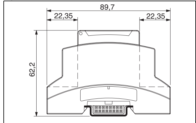
Figure 6 BC...U22, side view
