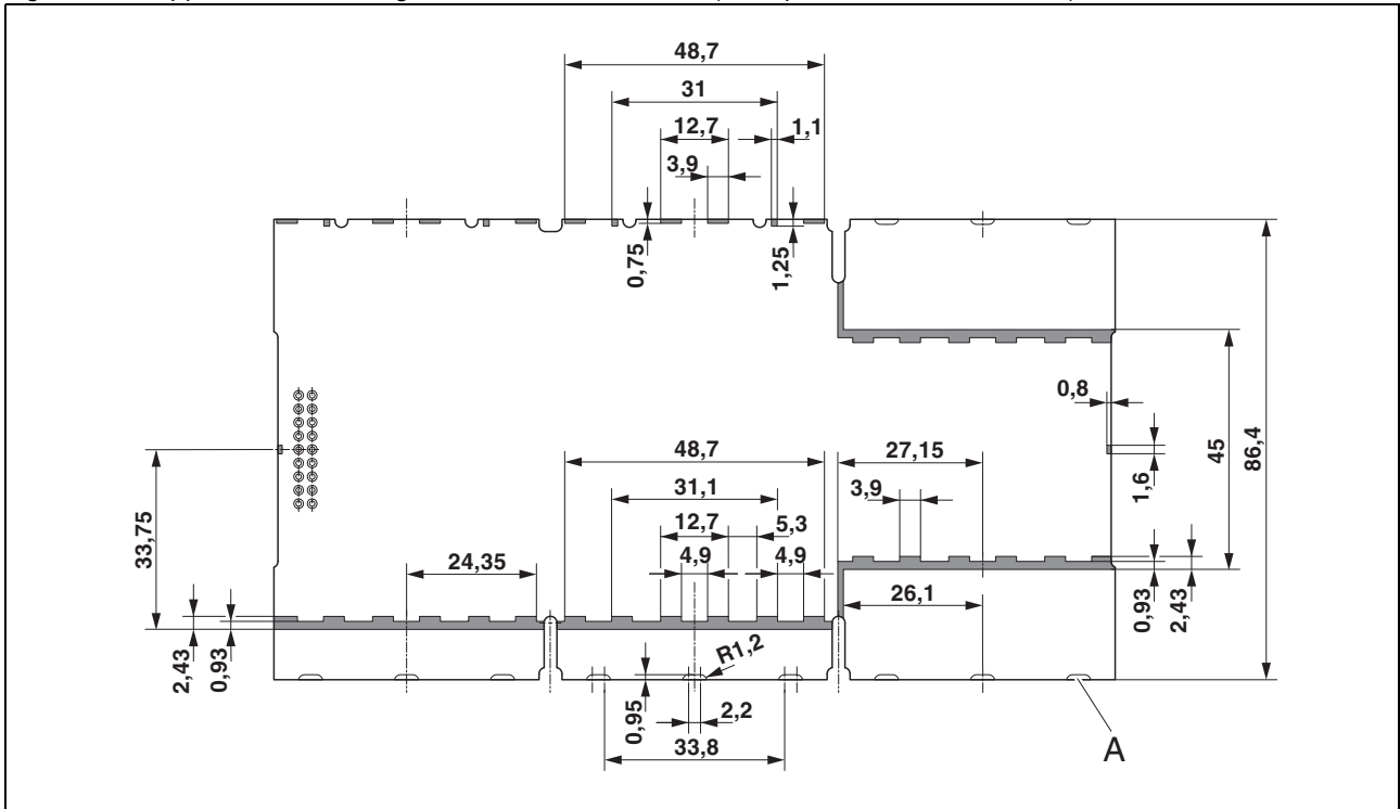
Figure 44 Upper side – mounting side of BC modular 161,6 (example BC 161,6 OT 010122)
