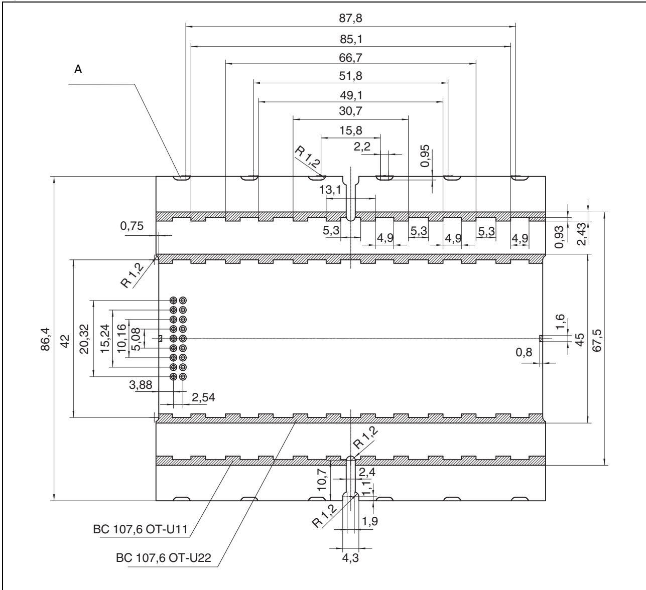
Figure 21 Dimensions of PCB 1 (BC 107,6) – upper side
