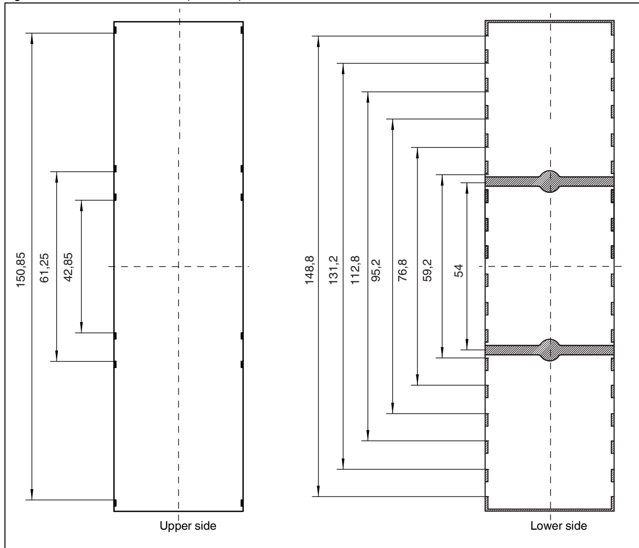
Figure 53 Dimensions of PCB 9 (BC 161,6)
