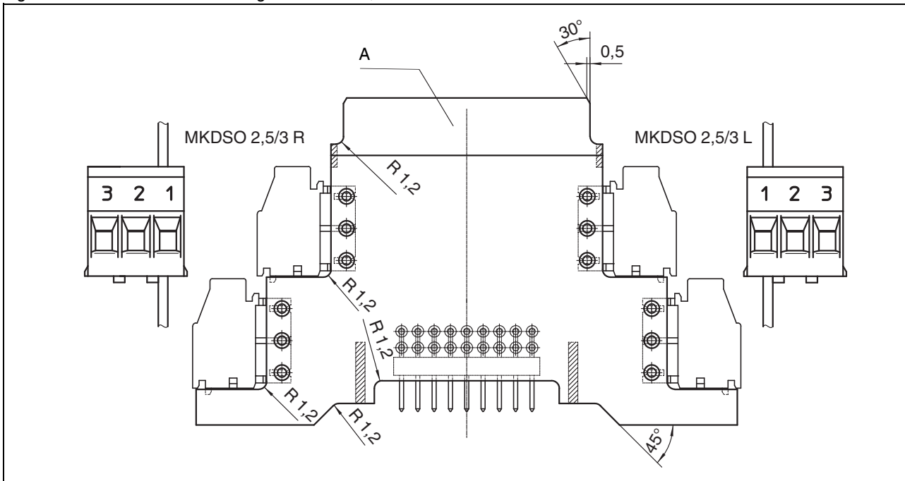
Figure 10 Lower side – soldering side of BC 17,8
