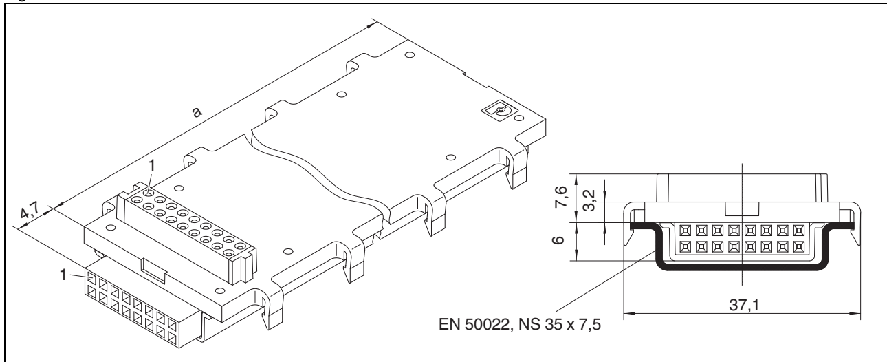
Figure 8 Dimensions of DIN rail connector HBUS and DIN rail NS 35
