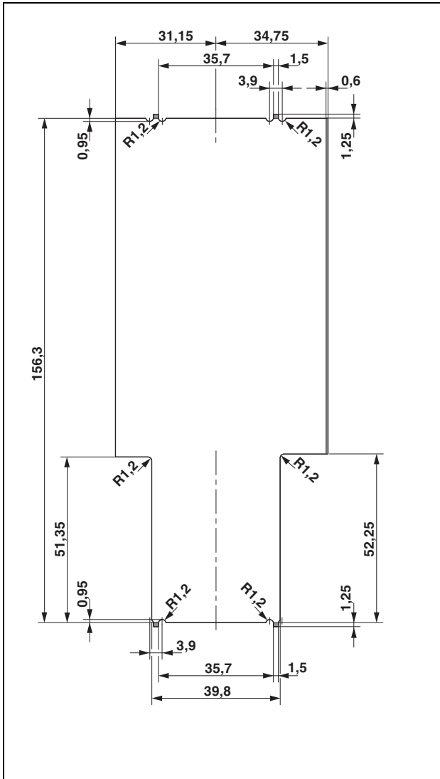
Figure 50 Dimensions of PCB 6 (example BC 161,6 OT 010122)
