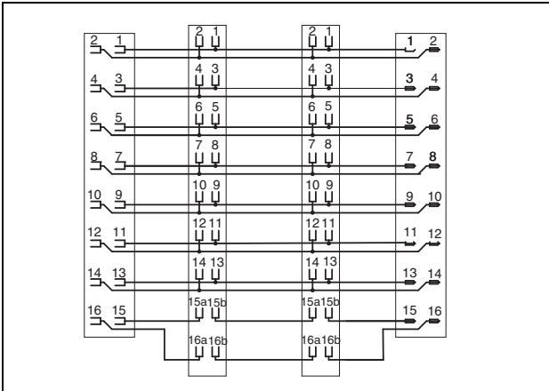
Figure 13 Circuit diagram for HBUS 53,6-16P-3S BK
