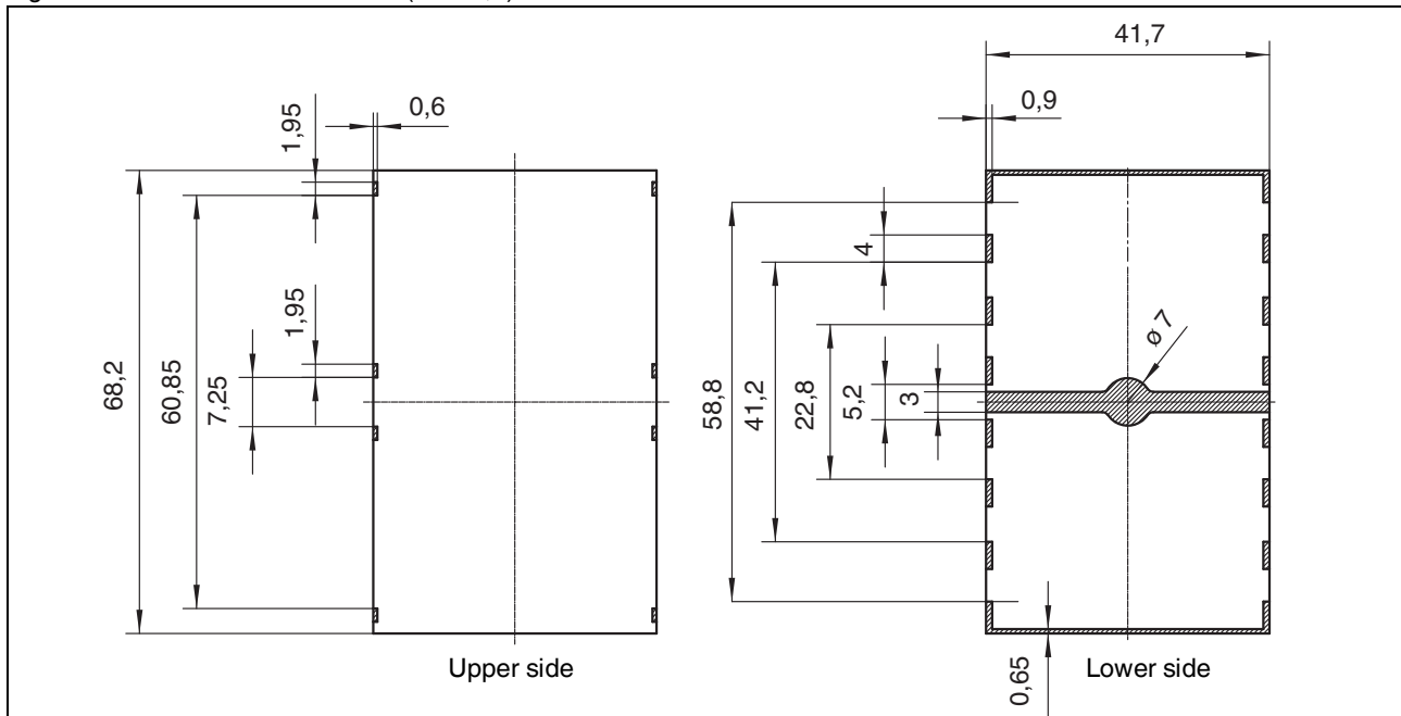
Figure 34 Dimensions of PCB 9 (BC 71,6)
