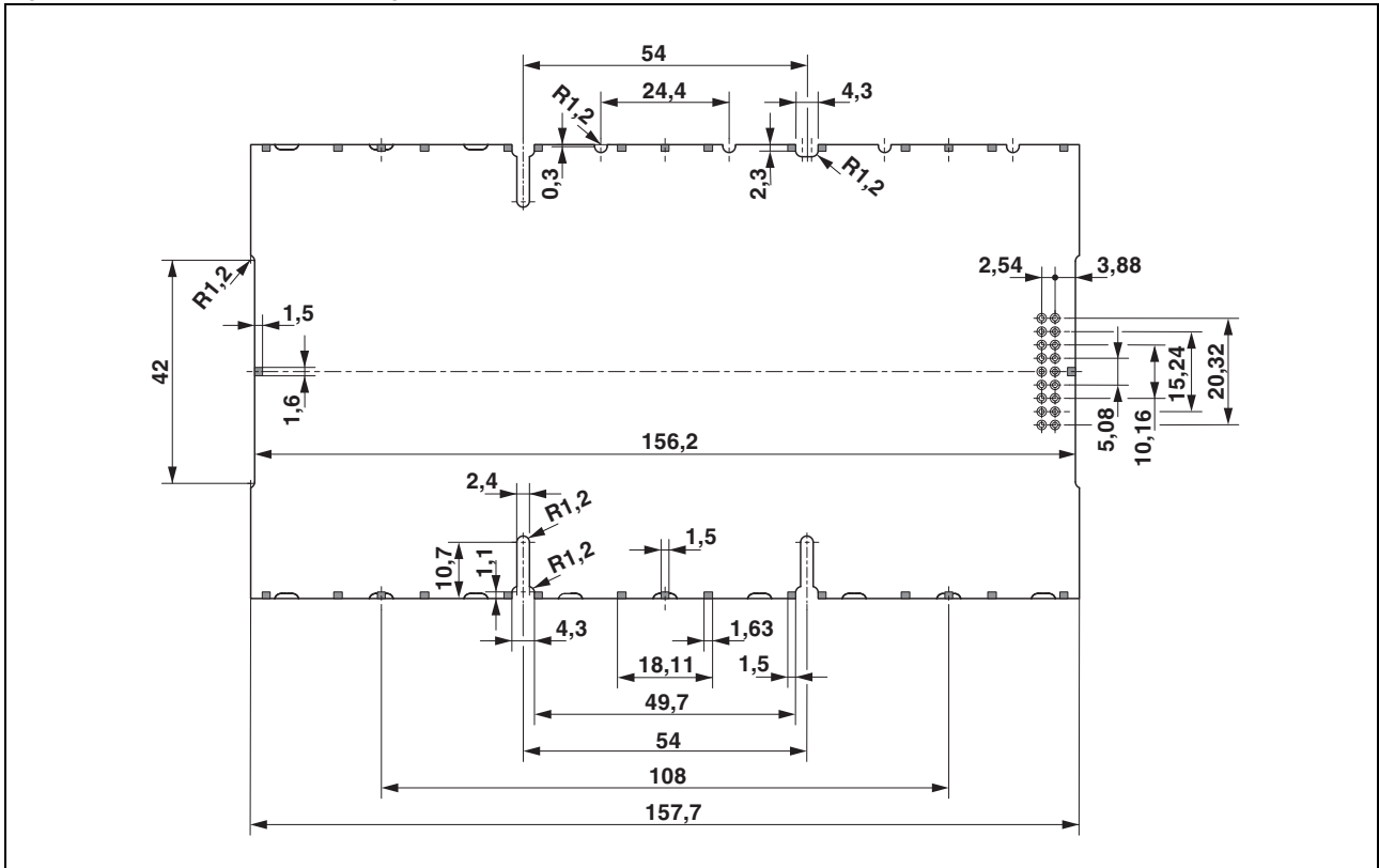
Figure 45 Lower side – soldering side of BC modular 161,6 (example BC 161,6 OT 010122)
