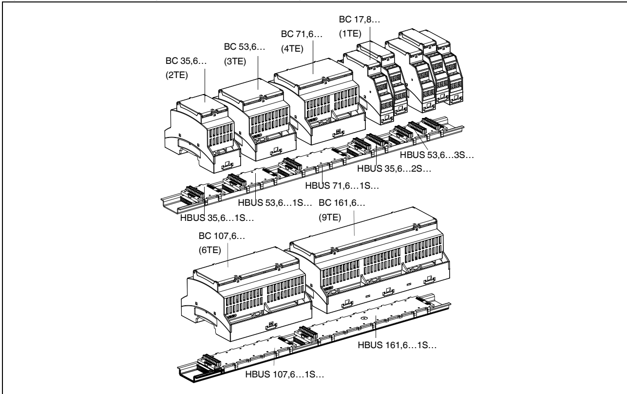
Figure 3 Overview of design widths with corresponding DIN rail connector HBUS
