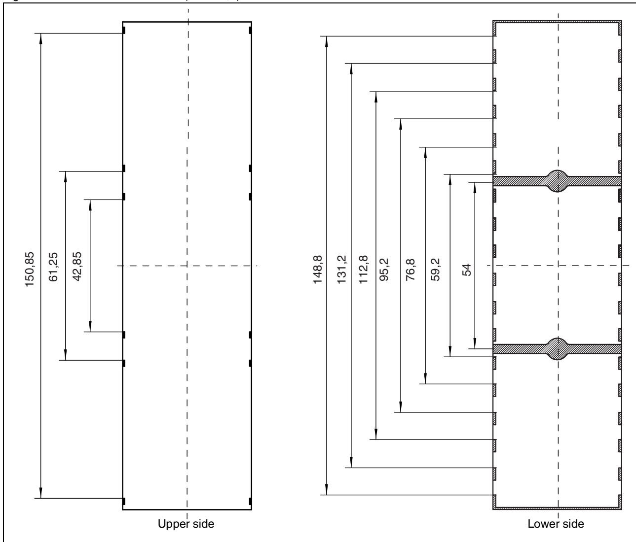
Figure 36 Dimensions of PCB 9 (BC 161,6)
