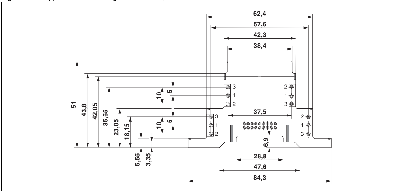
Figure 9 Upper side – mounting side of BC 17,8
