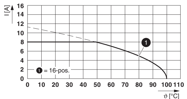
Figure 61 Derating
