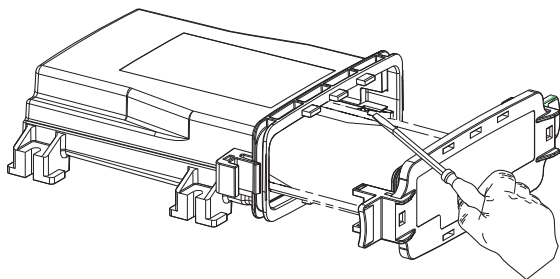
Figure 20 Board lock release
