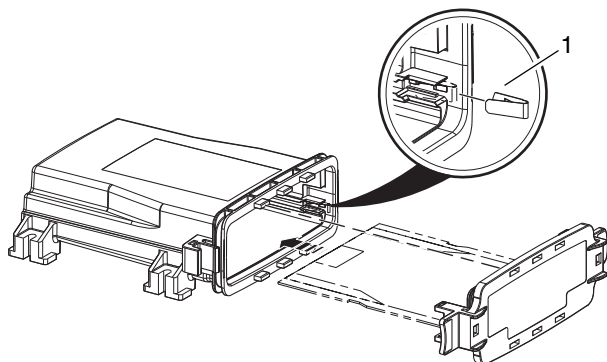
Figure 17 Board lock
