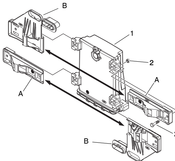
Figure 21 ECS-PM assembly
