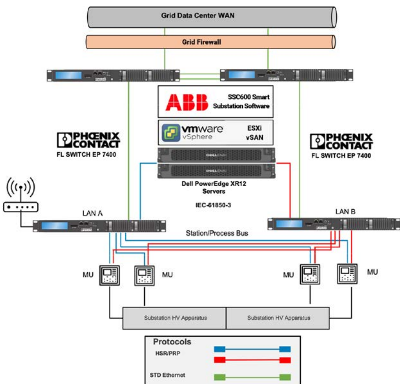
Figure 1. Physical Architecture of vPAC Platform
