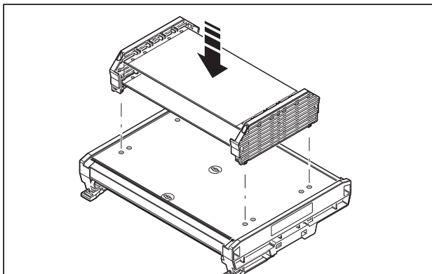
Figure 26 Attaching the lateral elements
