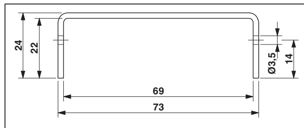
Figure 10 Dimensions of UM-PRO A/U N73 CM
