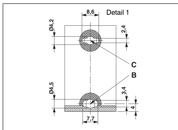
Figure 18 Cutouts for fixing
