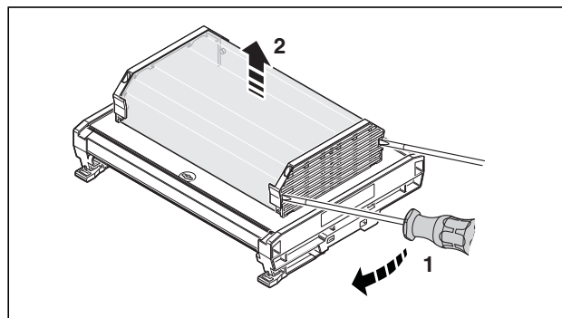
Figure 29 Removing the covering hood
