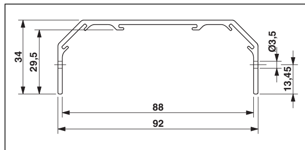
Figure 11 Dimensions of UM-PRO A/U 92 CM
