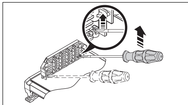
Figure 30 Removing the lateral elements
