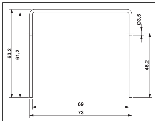
Figure 12 Dimensions of UM-PRO A/U 73 CM
