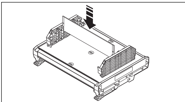
Figure 24 PCBs, vertical
