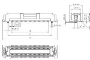
図1 (0.635 MV)
