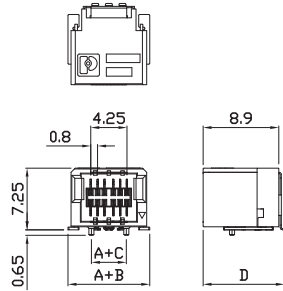
図4 (0.8 FH/FH-SH)
