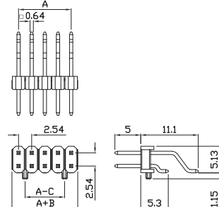
図14 (FQ2.54 PH)
