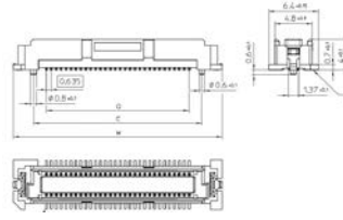
図2 (0.635 FV)
