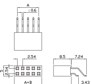
図15 (FQ2.54 SH)
