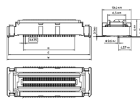
図2.5 (0.635 FV-F)
