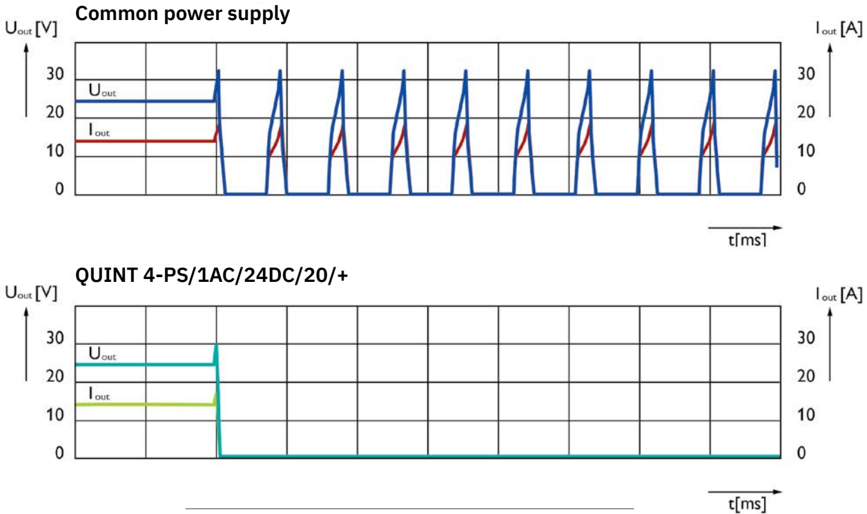
Figure 3: Overvoltage protection (OVP): unlike conventional power supplies, the QUINT Power Plus version (QUINT4-PS/1AC/24DC/20/+, switches the output off in the event of a voltage control fault, so it reliably protects consumers against damage resulting from failures.
