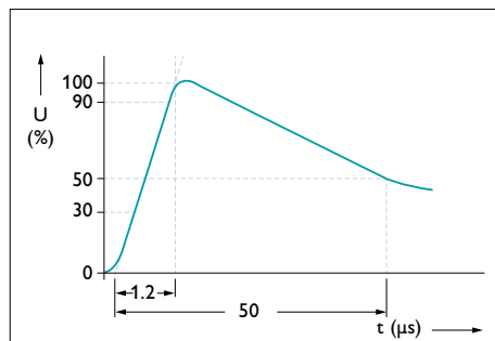
Fig. 20: Curve for a (1.2/50 \mu\text{s} ) voltage surge pulse
