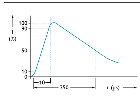
Fig. 21: Curve for a (10/350 \mu\text{s} ) surge current pulse
