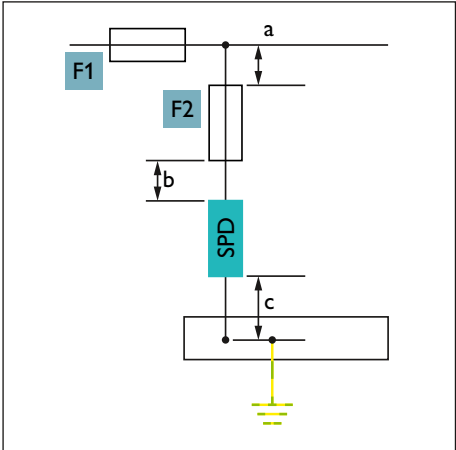
Fig. 53: Branch wiring
