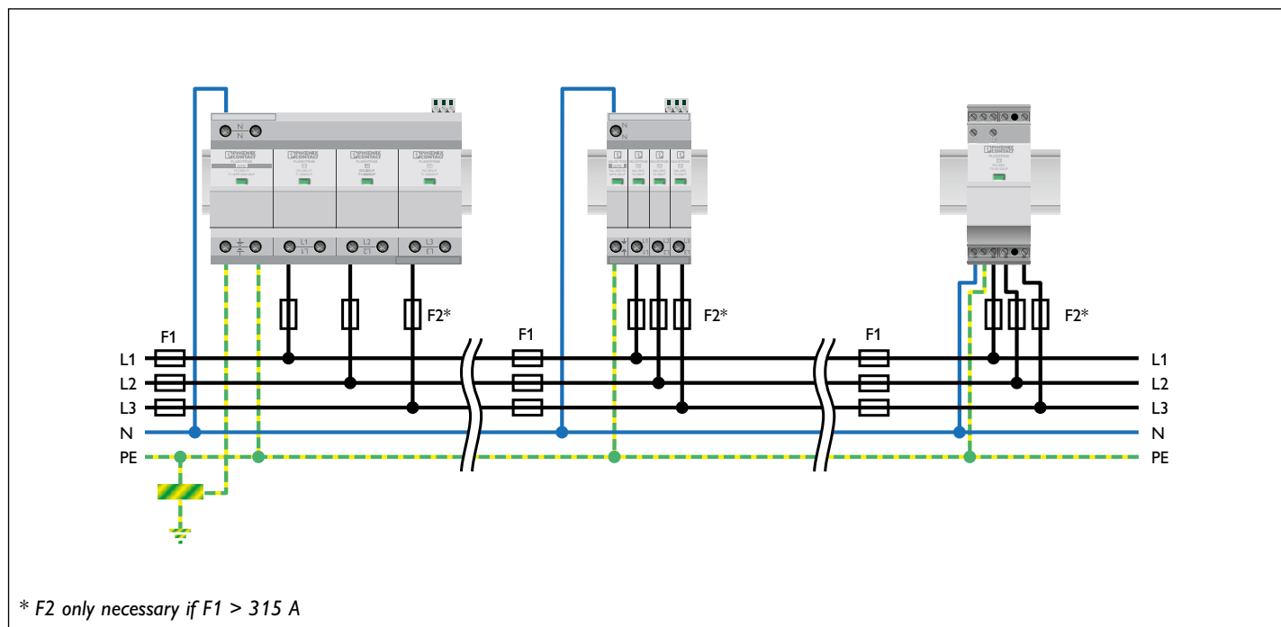
Fig. 58: Example connection of surge protective devices in a TN-S system
