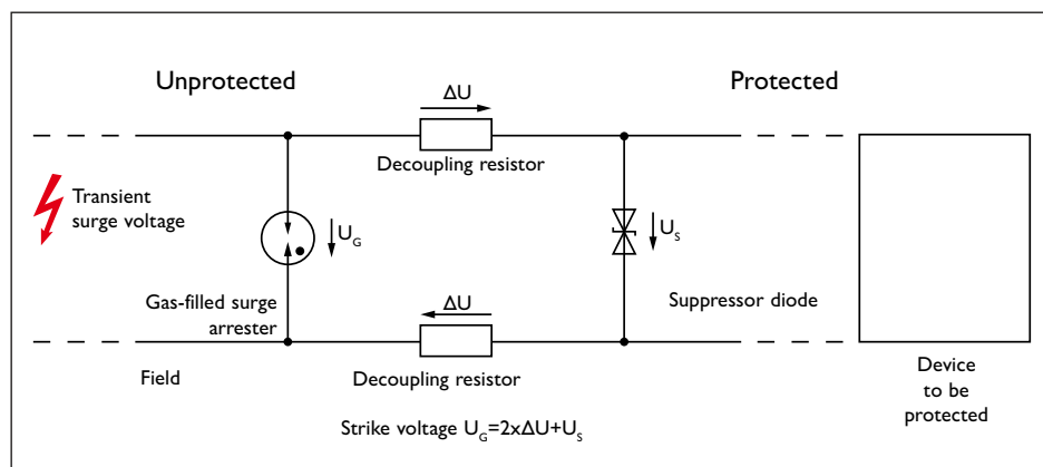
Fig. 76: Two-stage protective circuit
