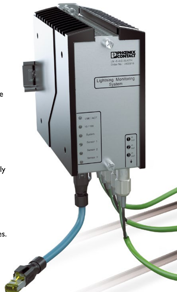
Fig. 33: The lightning monitoring system
