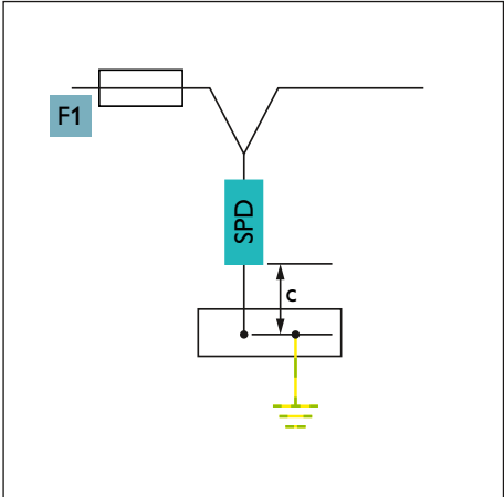
Fig. 54: V-wiring
