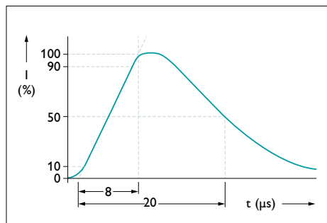
Fig. 19: Curve for a (8/20 \mu\text{s} ) surge current pulse
