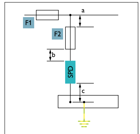
Fig. 53: Branch wiring
