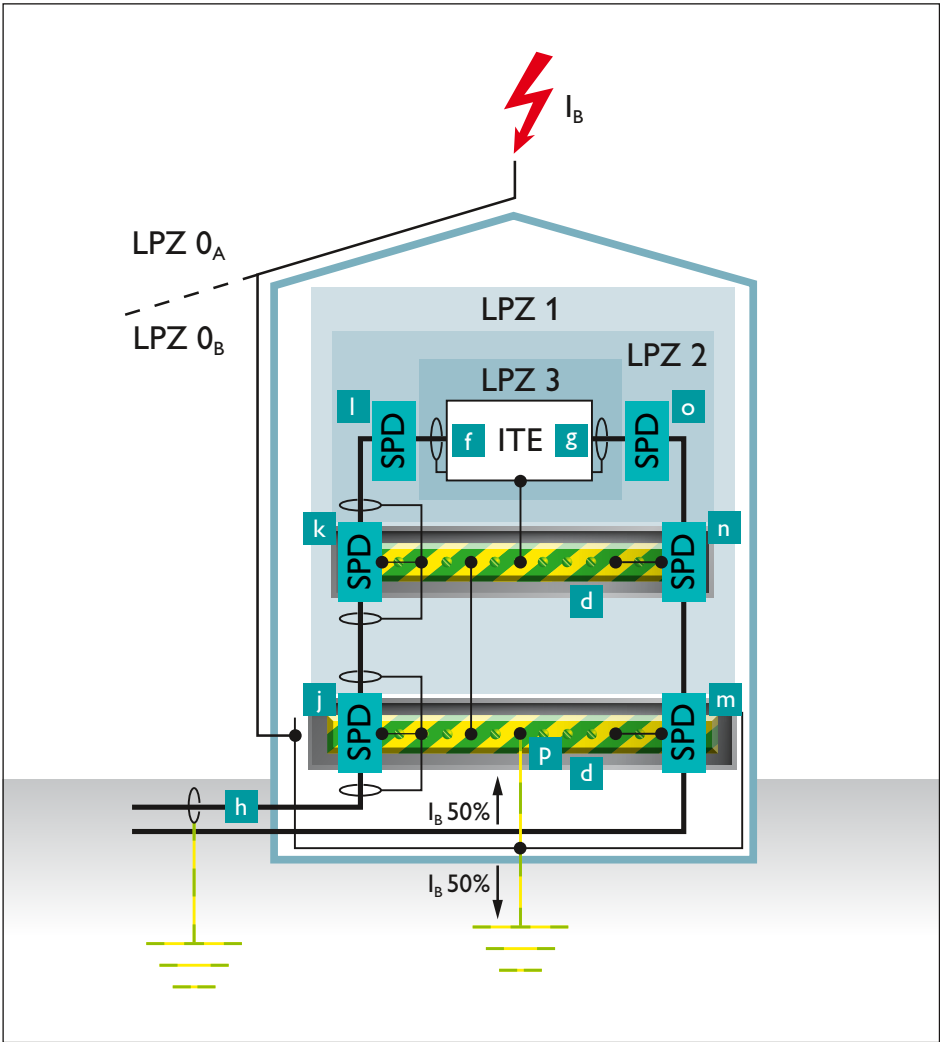
Fig. 81: Zone concept in accordance with IEC 61643-22 [16]
