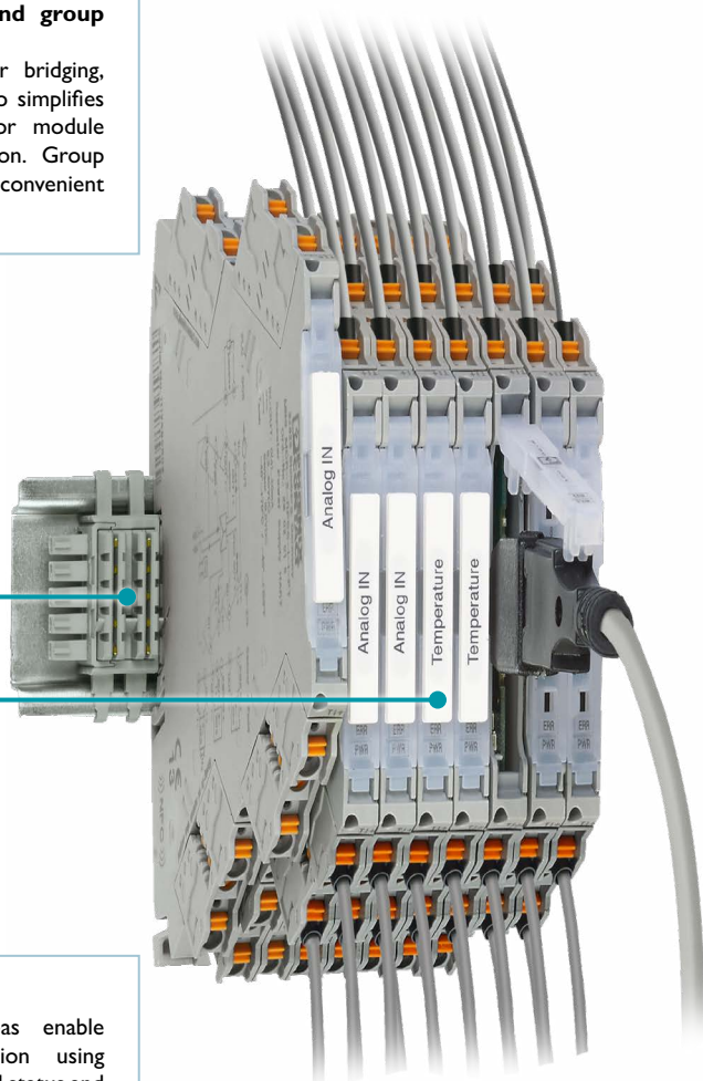
Measure signals during operation, without disconnecting the current loops
