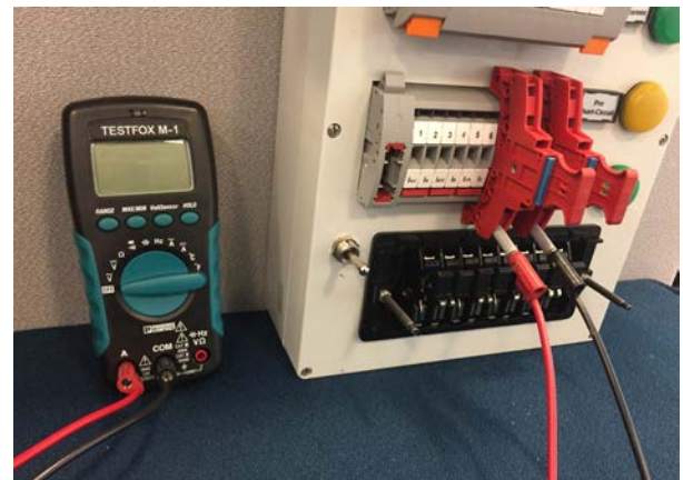
Figure 8: FAME test probes used for voltage readings.
