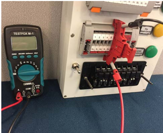
Figure 10: Test plug inserted, and current reading obtained.
