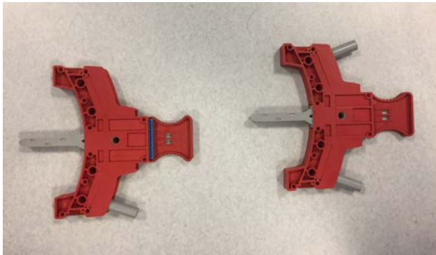
Figure 5: FAME test probes used for voltage with a bridge (left) and used for current (right).
