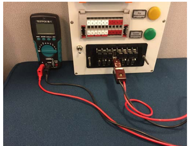
Figure 3: Duck bill attached to ammeter prior to inserting into test point.
