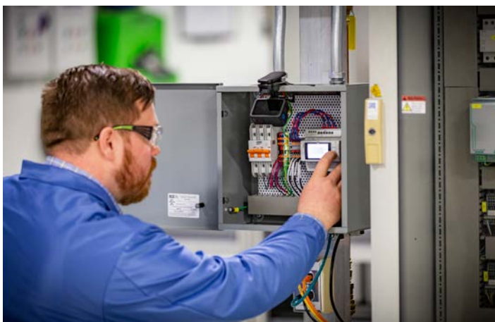
Figure 2: Basic energy meters, like the Phoenix Contact EMpro, can measure and collect system conditions like voltage, current, and power.
