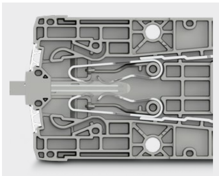
L-plate – early switching point
