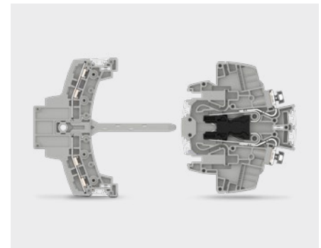
FAME 3 auxiliary contact for status recognition
