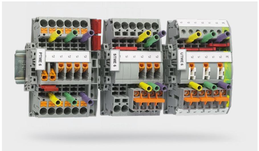
Test-disconnect terminal blocks with various connection technologies
