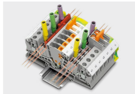
Transformer terminal block with six function shafts
