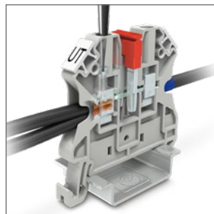
Terminal block with UT screw connection
