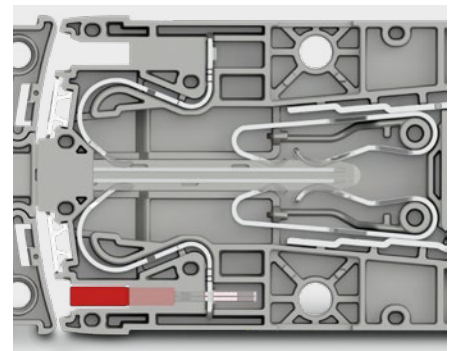
S-plate – late switching point
