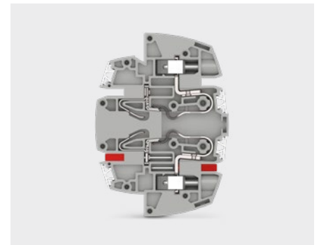
FAME 1 plug-in test socket
