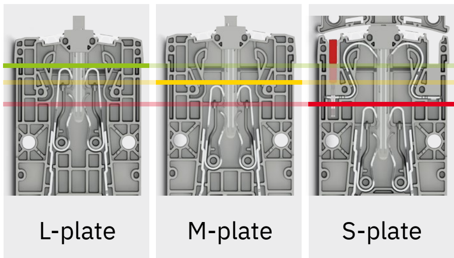
Switching points of the FAME 3 RACK plug-in test system
