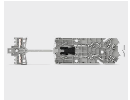
Auxiliary contact for status detection
