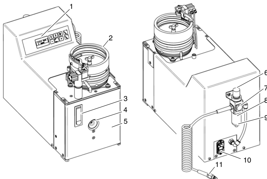
Figure 2-1 Operating components
