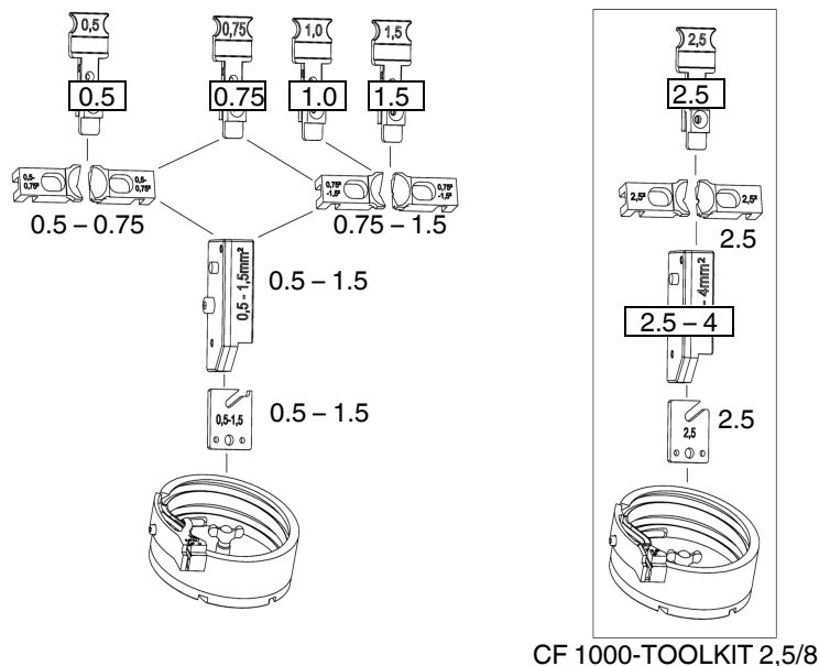
Figure 3-1 Example of CF 1000-1,5 (value in mm²)
