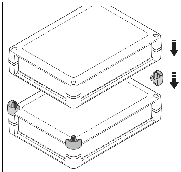
Figure 10 Mounting UCS CS... stacking adapters
