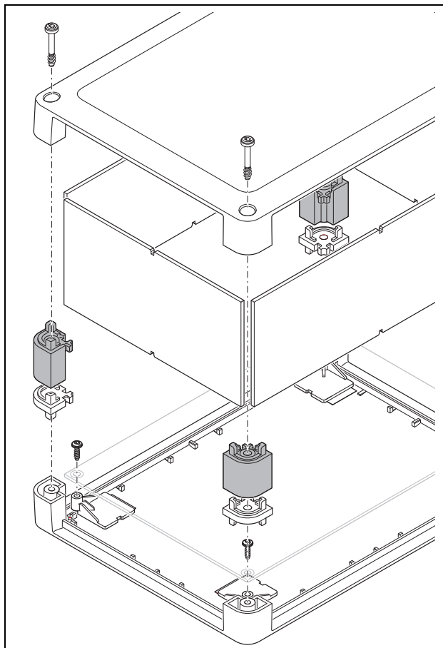
Figure 9 UCS HAC... height adapters
