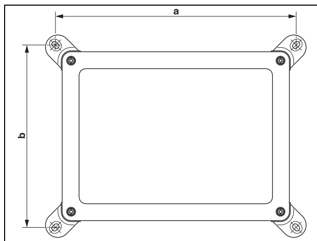
Figure 15 UCS WM-B... wall bracket, drilling diagram
