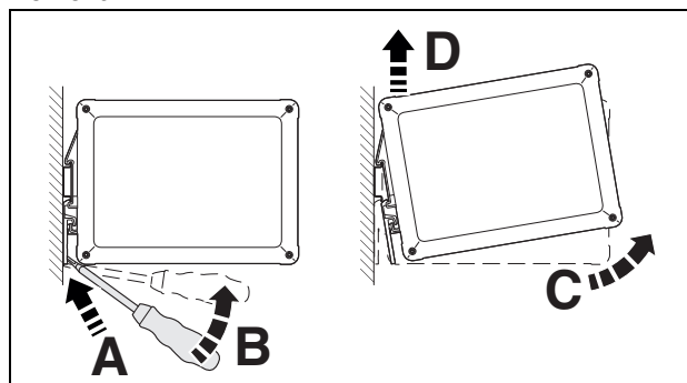
Figure 22 Removal
