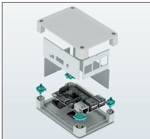
Figure 1 Housing components
