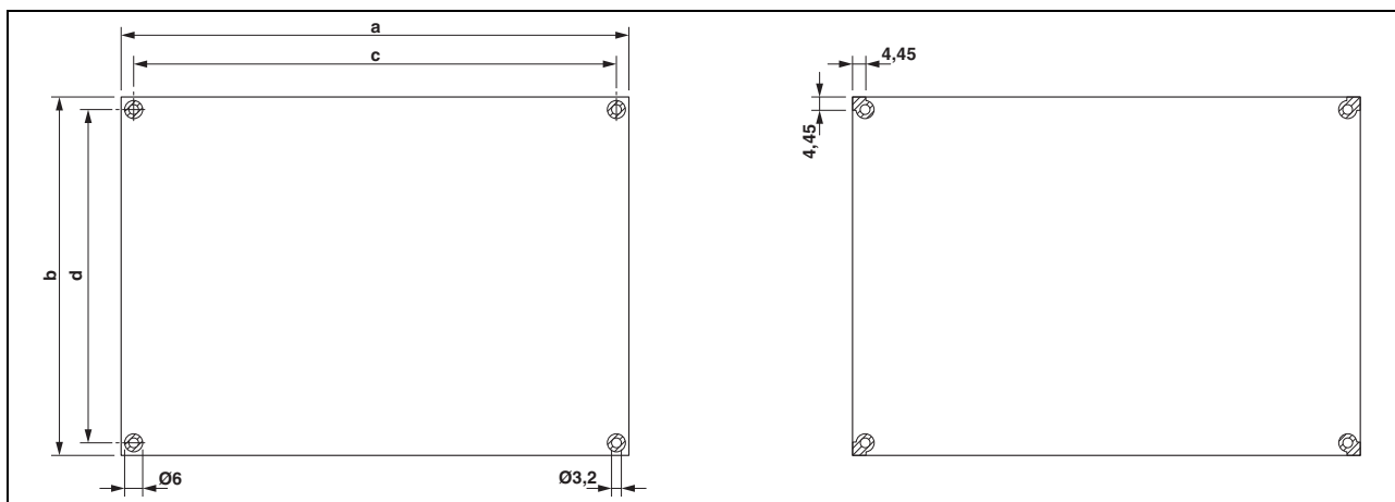
Figure 7 Maximum PCB dimensions
