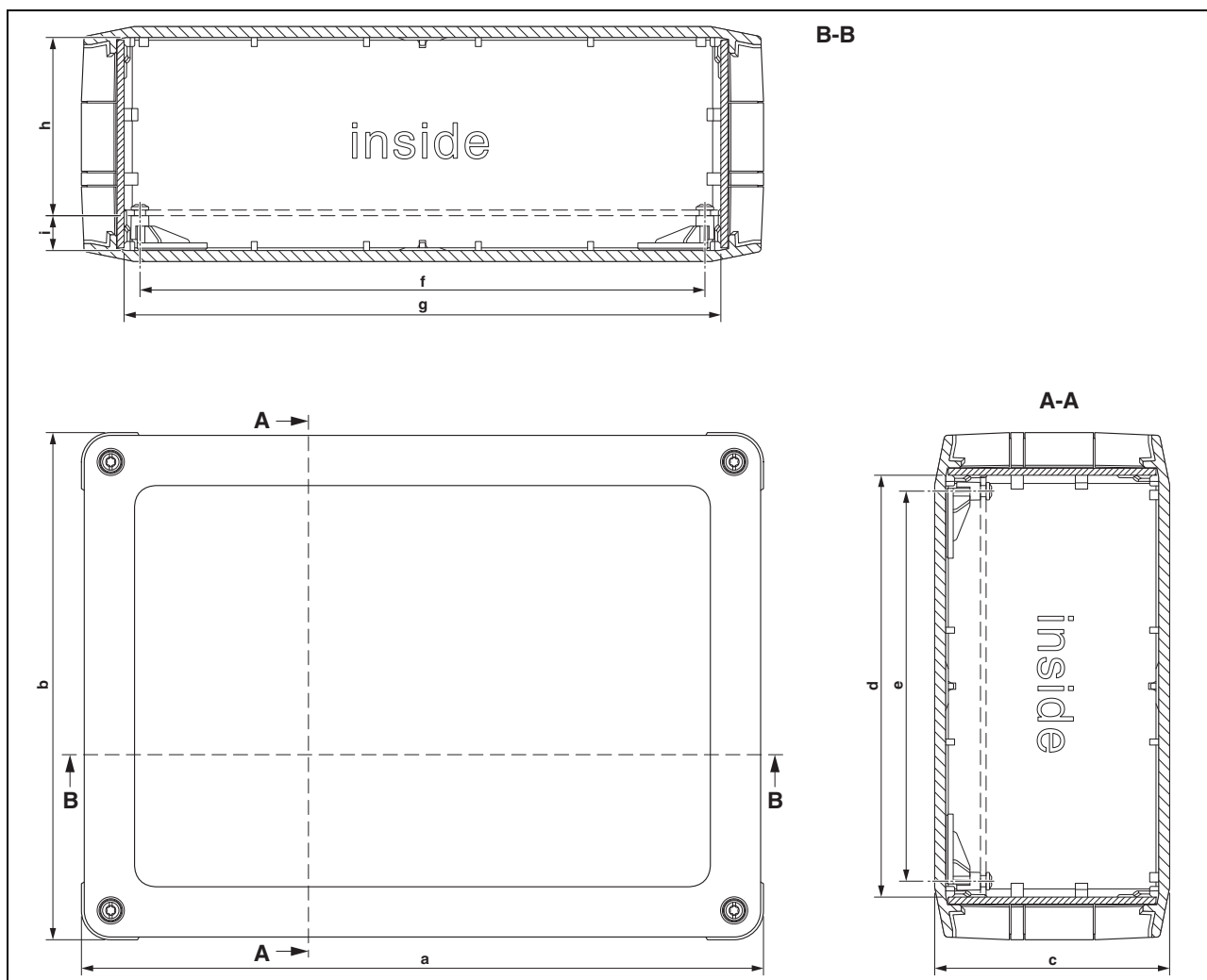
Figure 3 Housing dimensions
