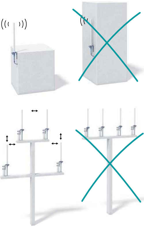
It is best to install the antennas above each other on a pole.
