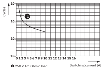
Electrical service life
