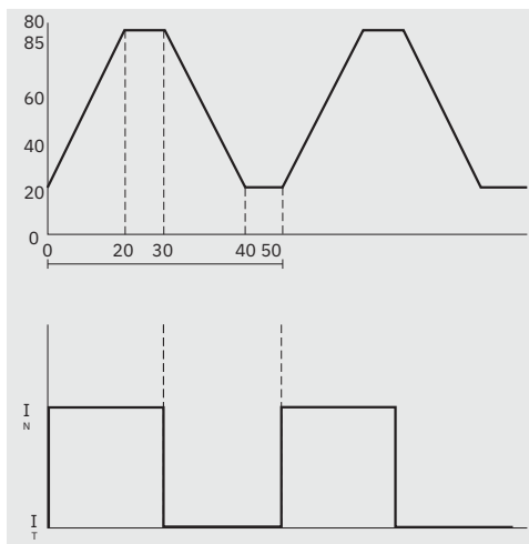
Current and temperature in relation to time t_T
