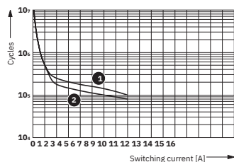
Electrical service life
