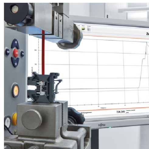
Absorption of tensile force at a 6 mm² screw terminal block
