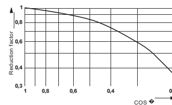
Service life reduction factor
