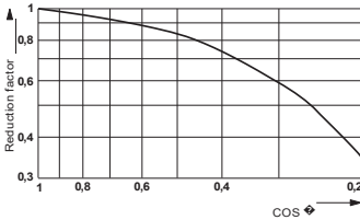
Service life reduction factor
