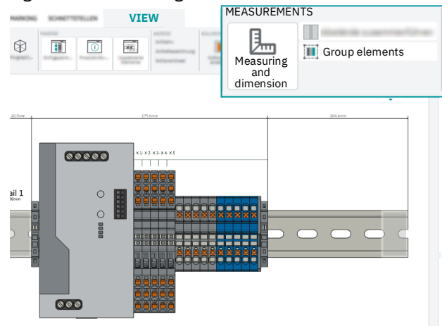
Figure 5 Measuring and dimension
